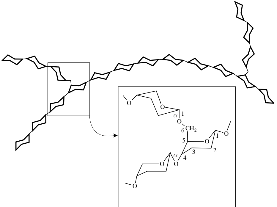
Amylopectine
