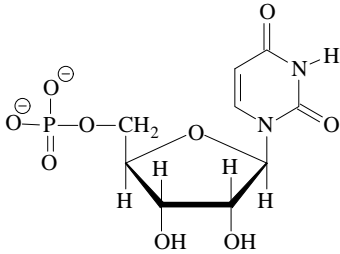
Uridylyl [U]
