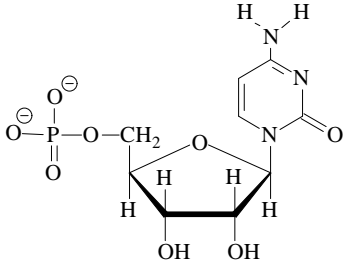
Cytidylyl [C]
