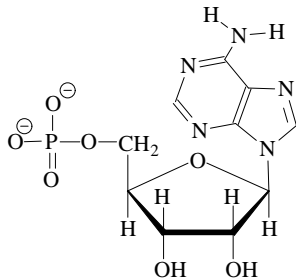
Adenylyl [A]
