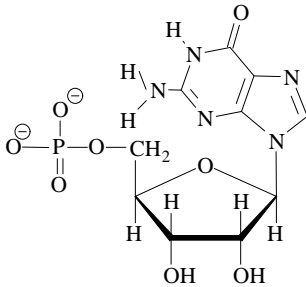
Guanylyl [G]
